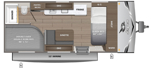
172DB/172DBW SPORT
